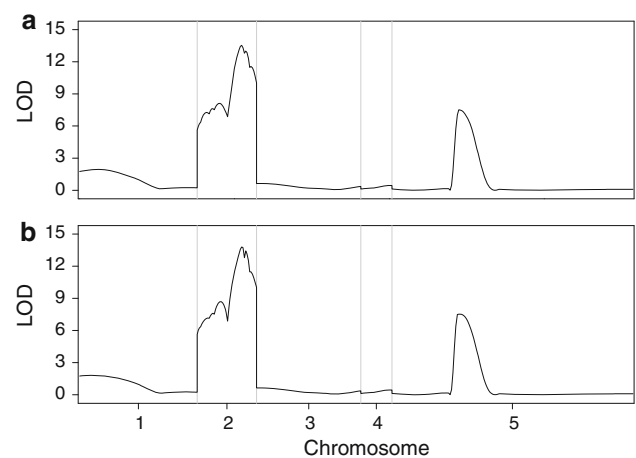
Fig. 1 The LOD profiles for the female sterility (binary) trait of wheat. a The upper panel shows the LOD profile for the heterogeneous variance model; b the lower panel shows the LOD profile for the mixture model. The chromosomes are separated by the vertical gray reference lines
